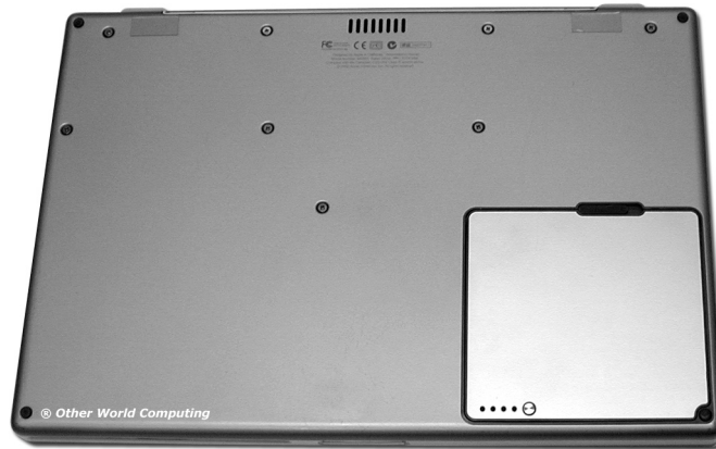
Bottom side of a PowerBook G4/500MHz. Some systems will look different and have screws in different locations, although the objective is the same.
